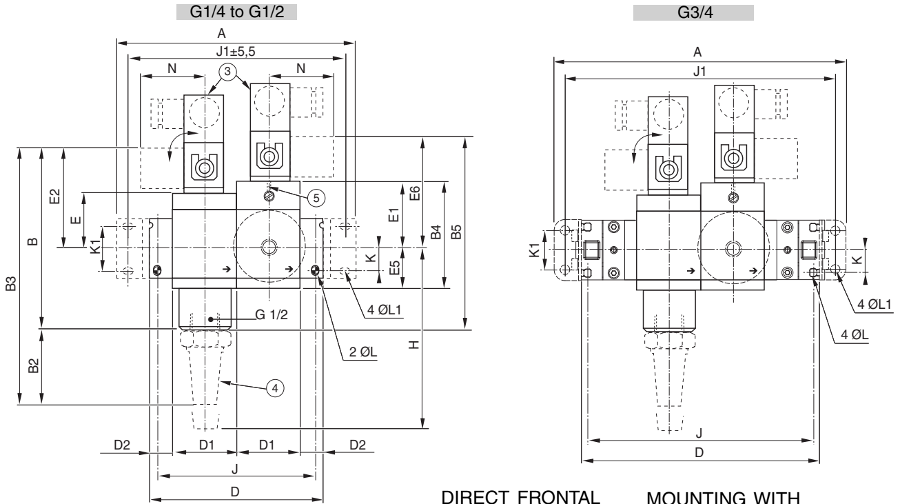
DIRECT FRONTAL MOUNTING ① OR LATERAL (G3/4)
