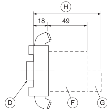
SUBBASE + SEQUENCER
