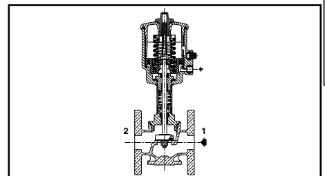
NC function, entry under the disc
